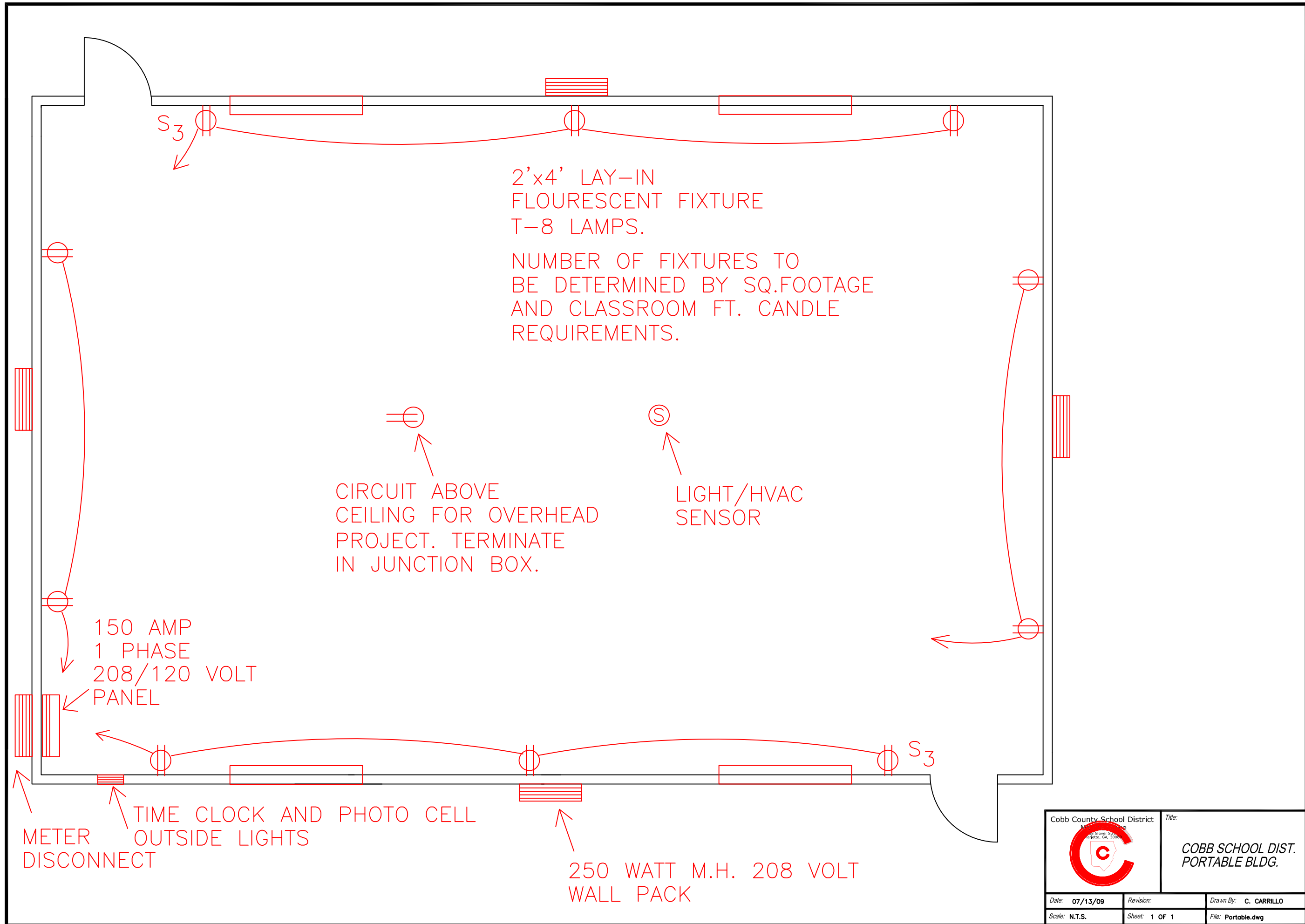
DRAWING "A"
