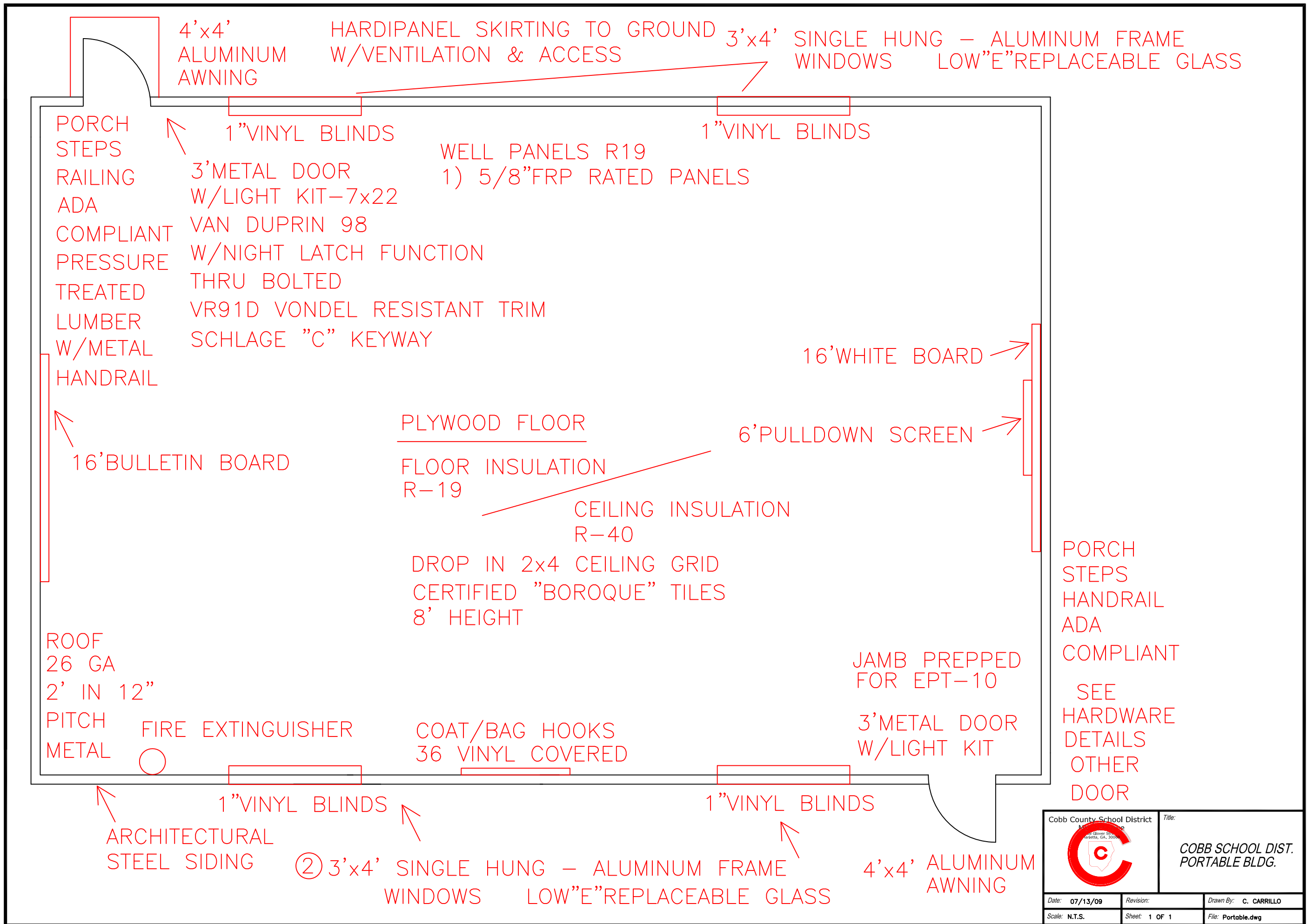
DRAWING "B"
