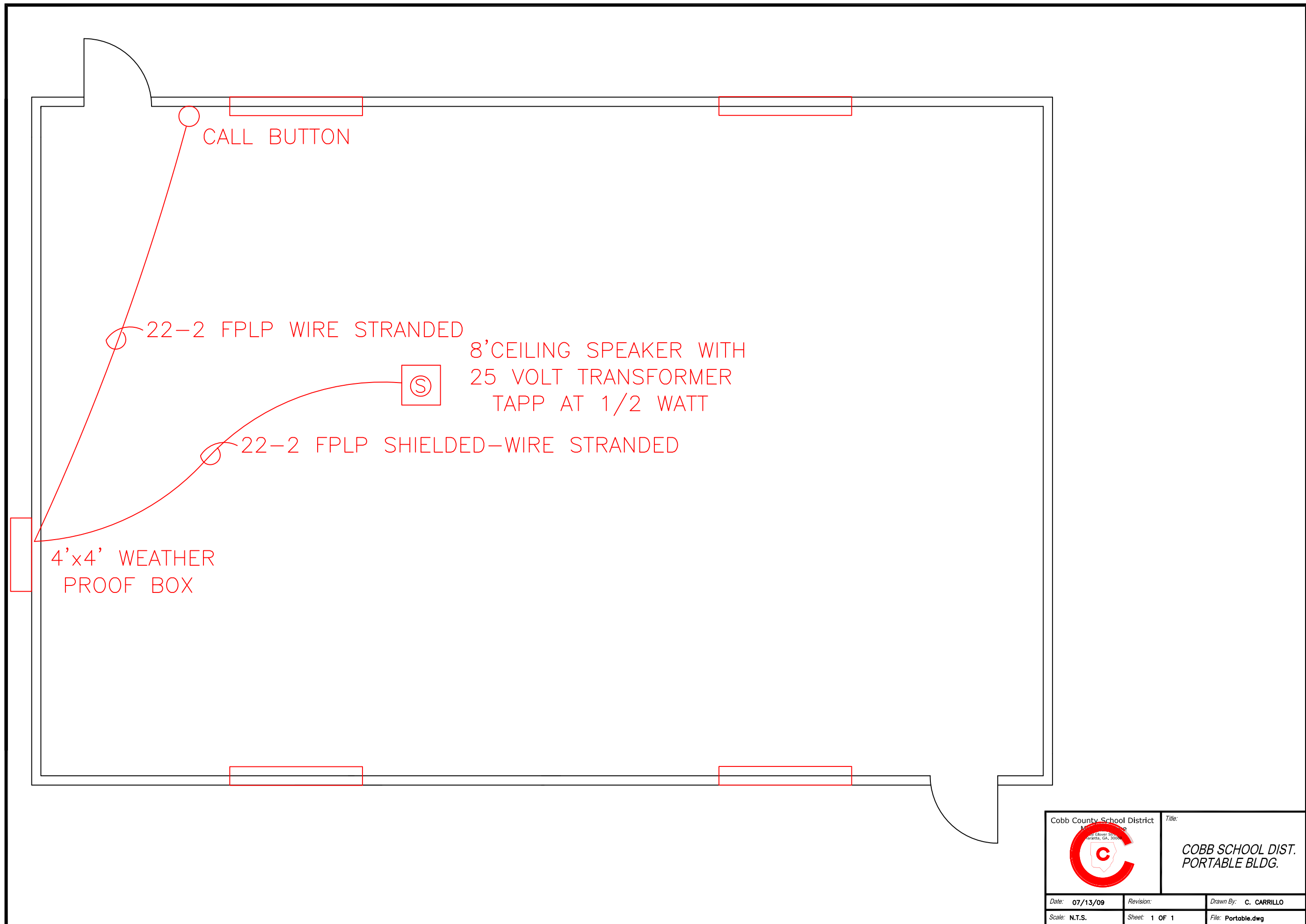
DRAWING "D"
